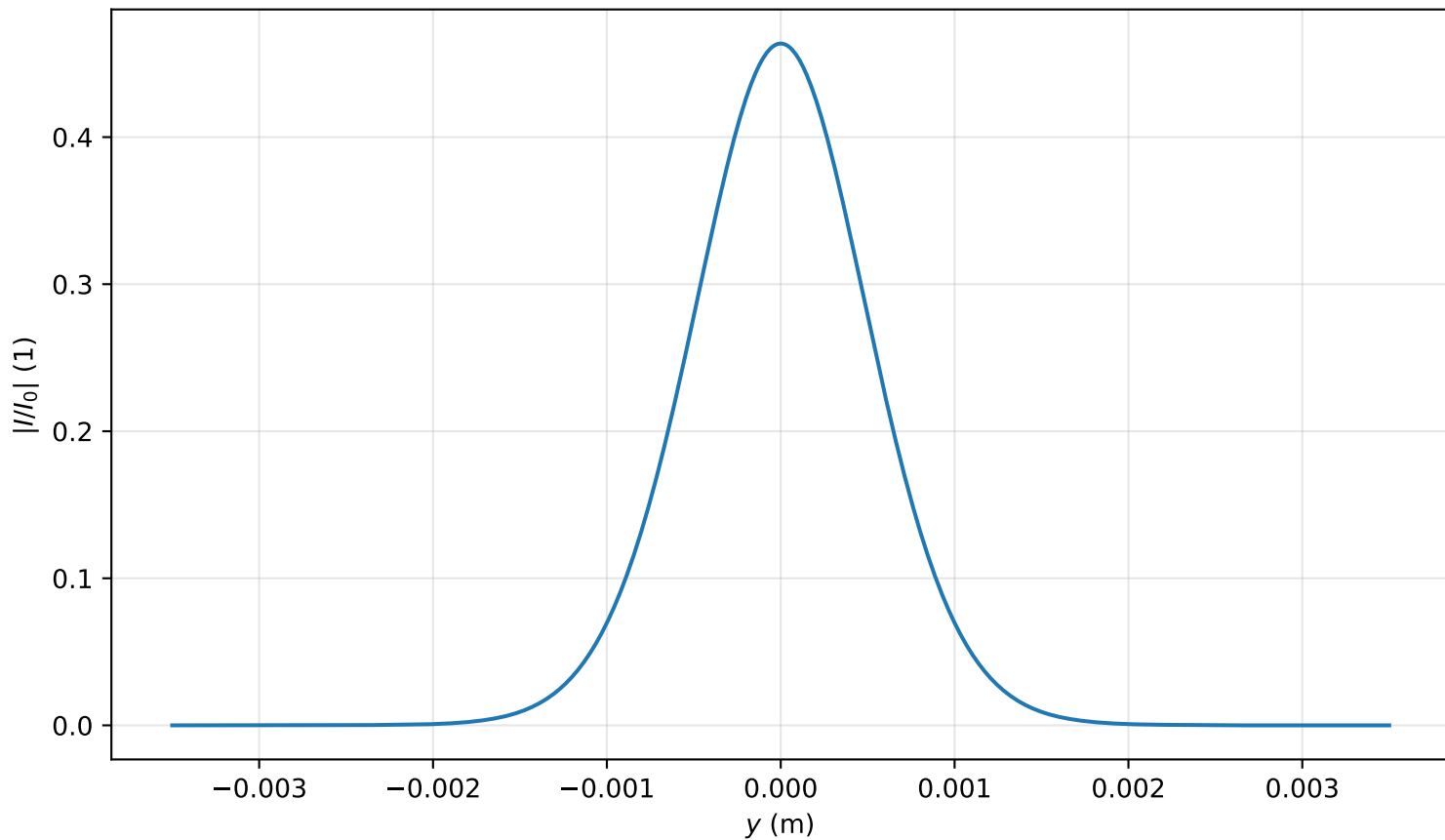
Intensity profile I(x=0, y, z=2.786)/I_0 , P_{in}=0.3P_{cr} , artificial time
